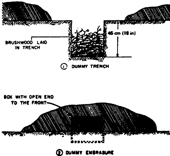
Figure 2-27. Dummy earthworks.
